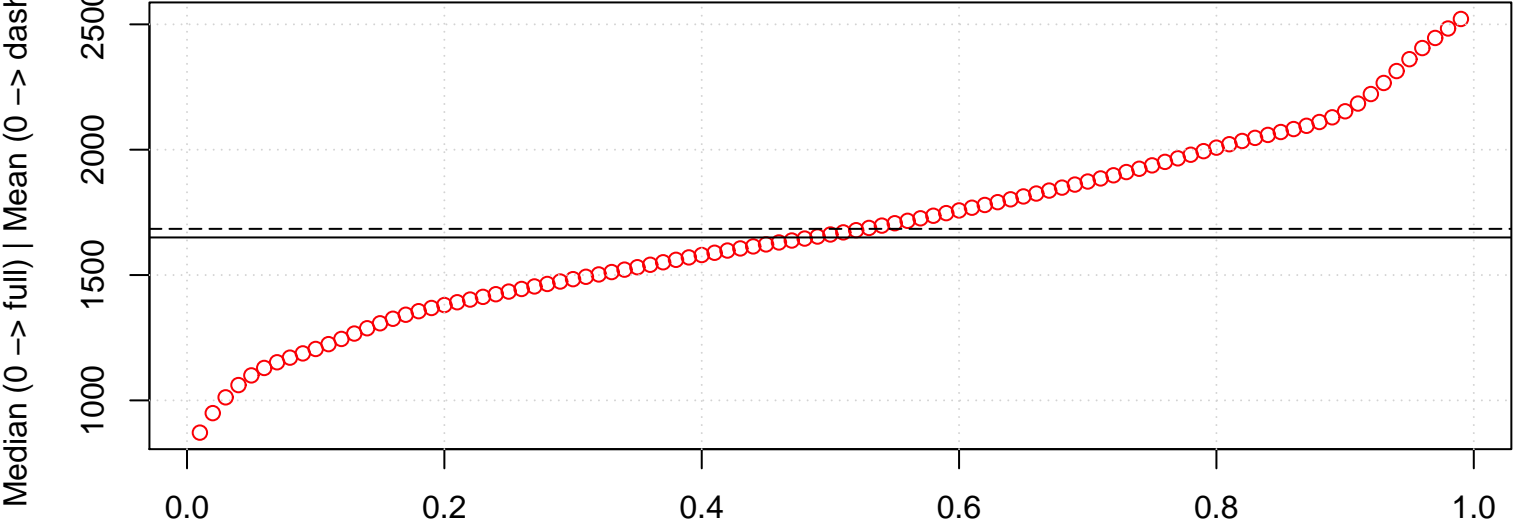
Harrell-Davis Quantiles
