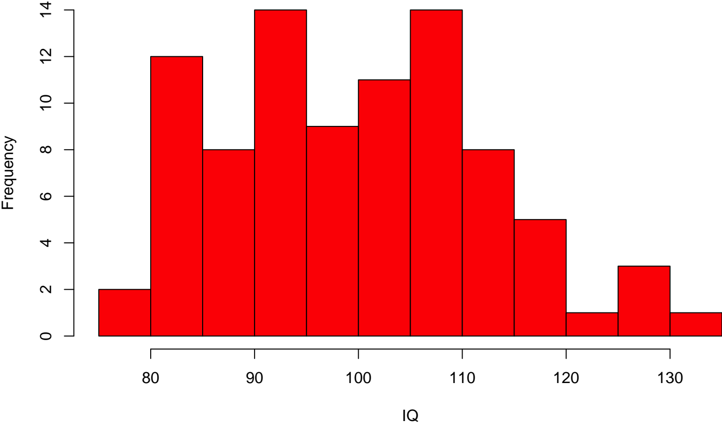
IQ/ GRADE Regression HISTOGRAM
