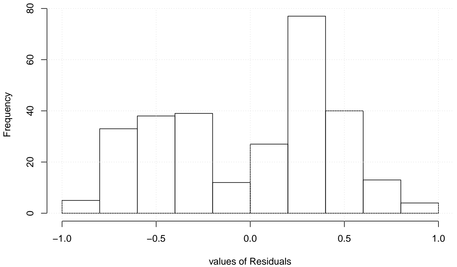
Residual Histogram
