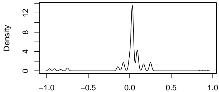
Kernel Density Plot of Residuals
