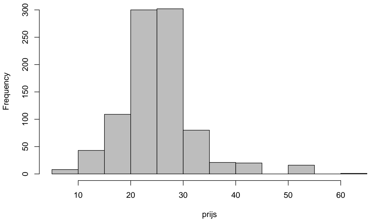
Histogram studio 100 default bins
