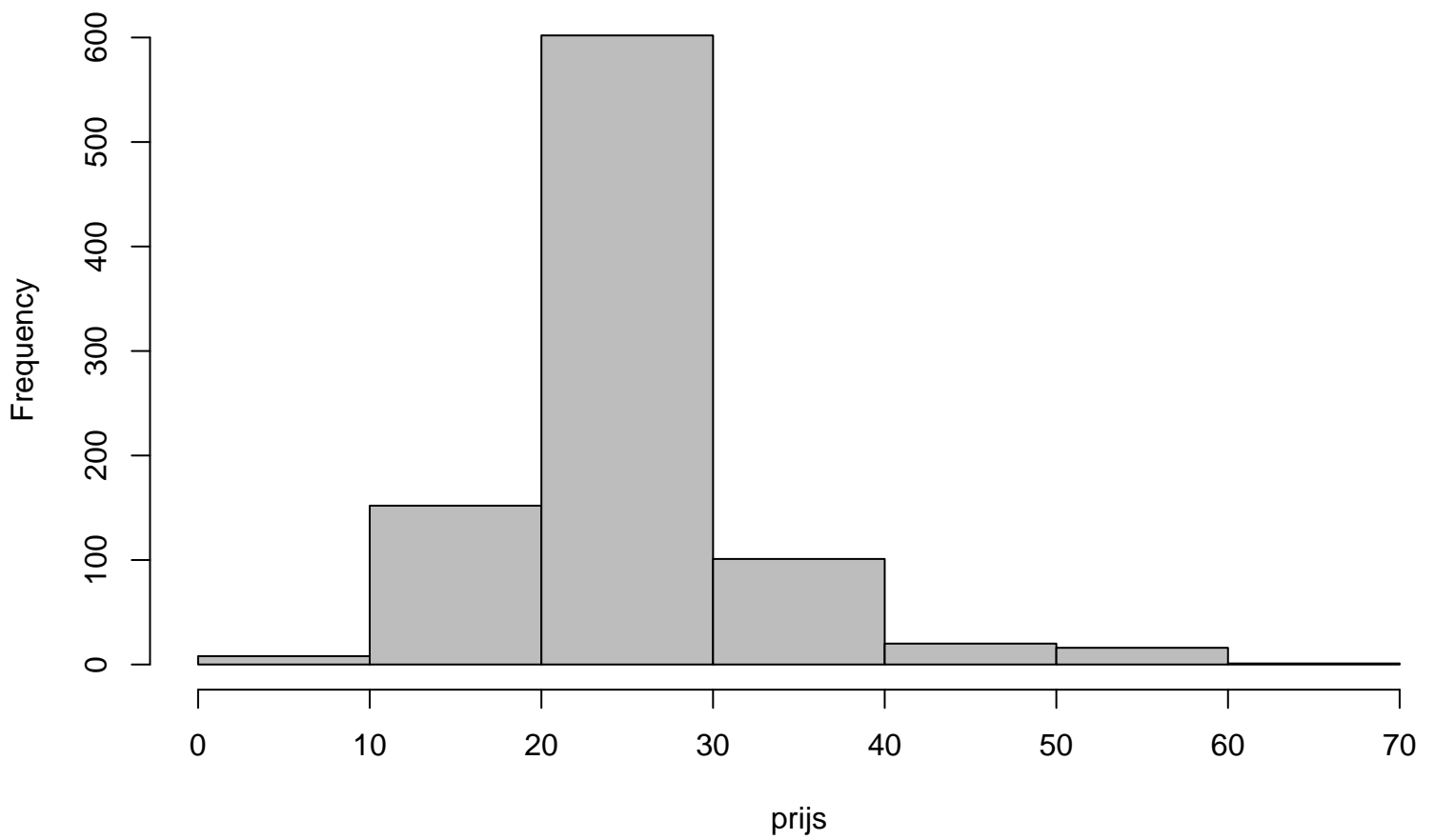
Histogram studio 100 6 bins
