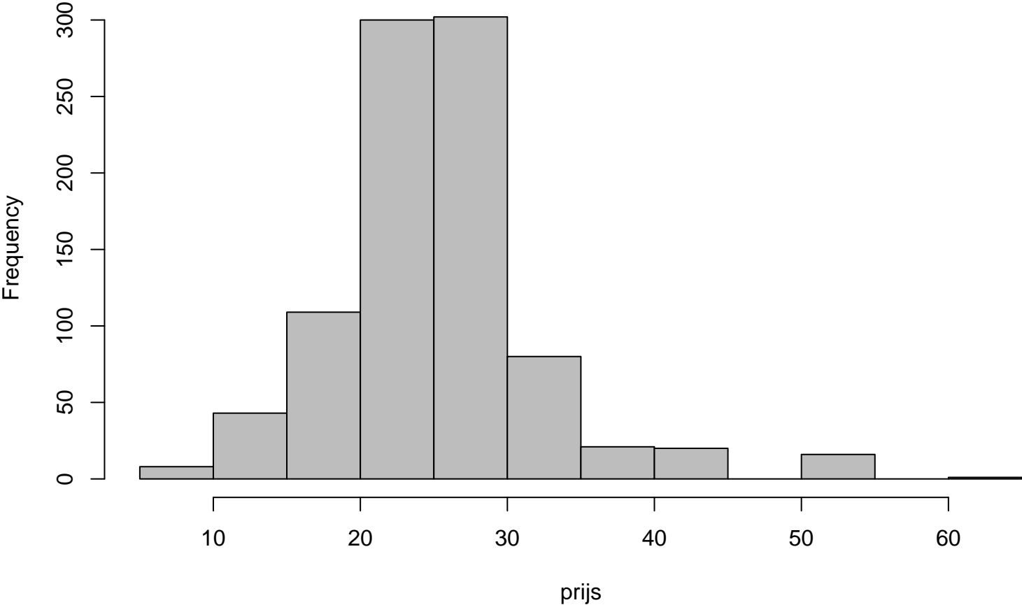
Histogram studio 100 14 bins
