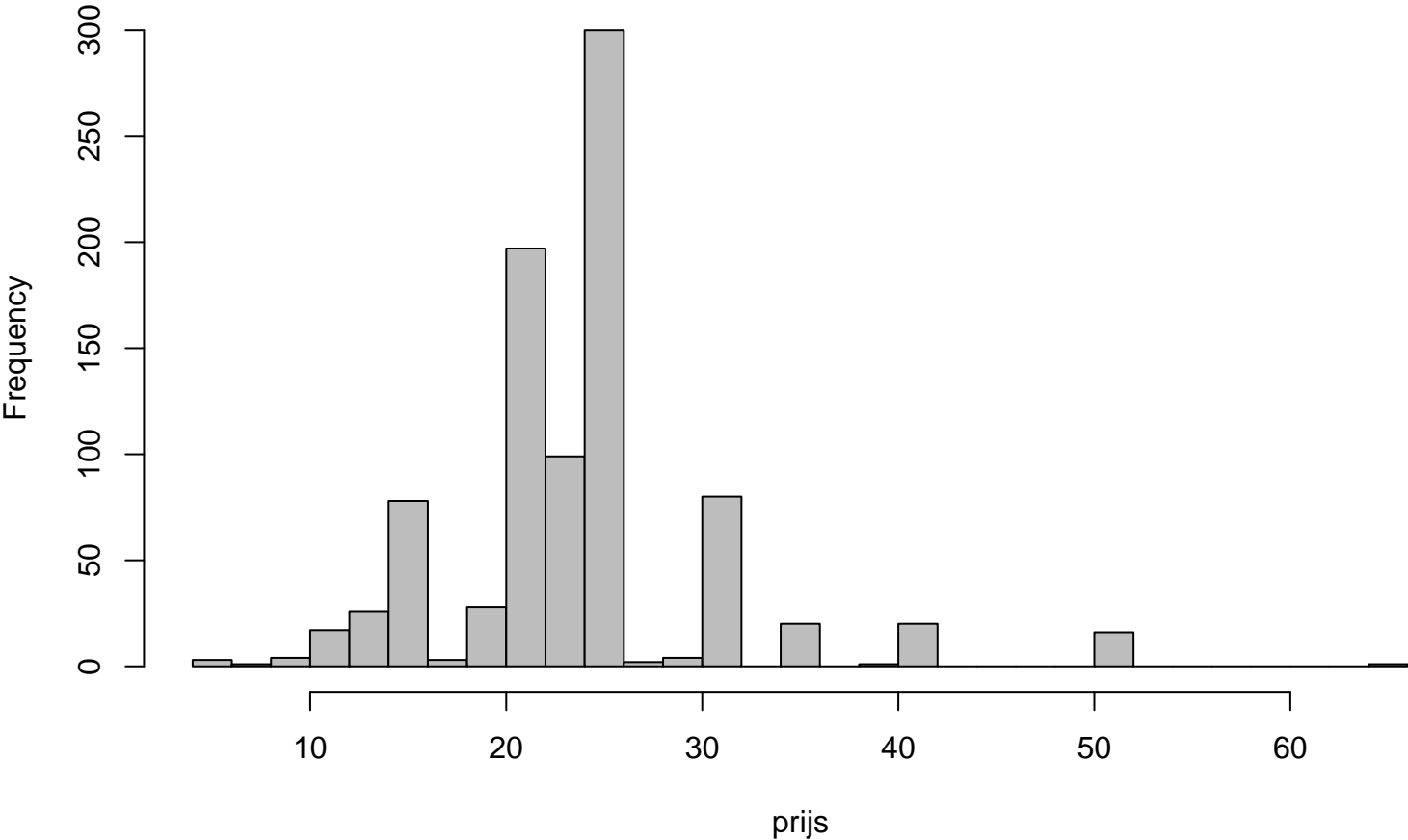
Histogram studio 100 24 bins
