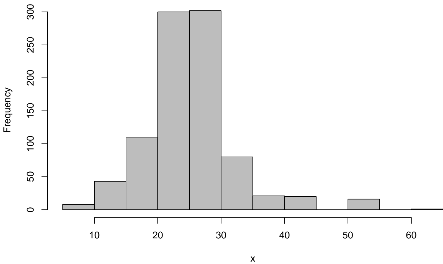
Histogram 12 bins
