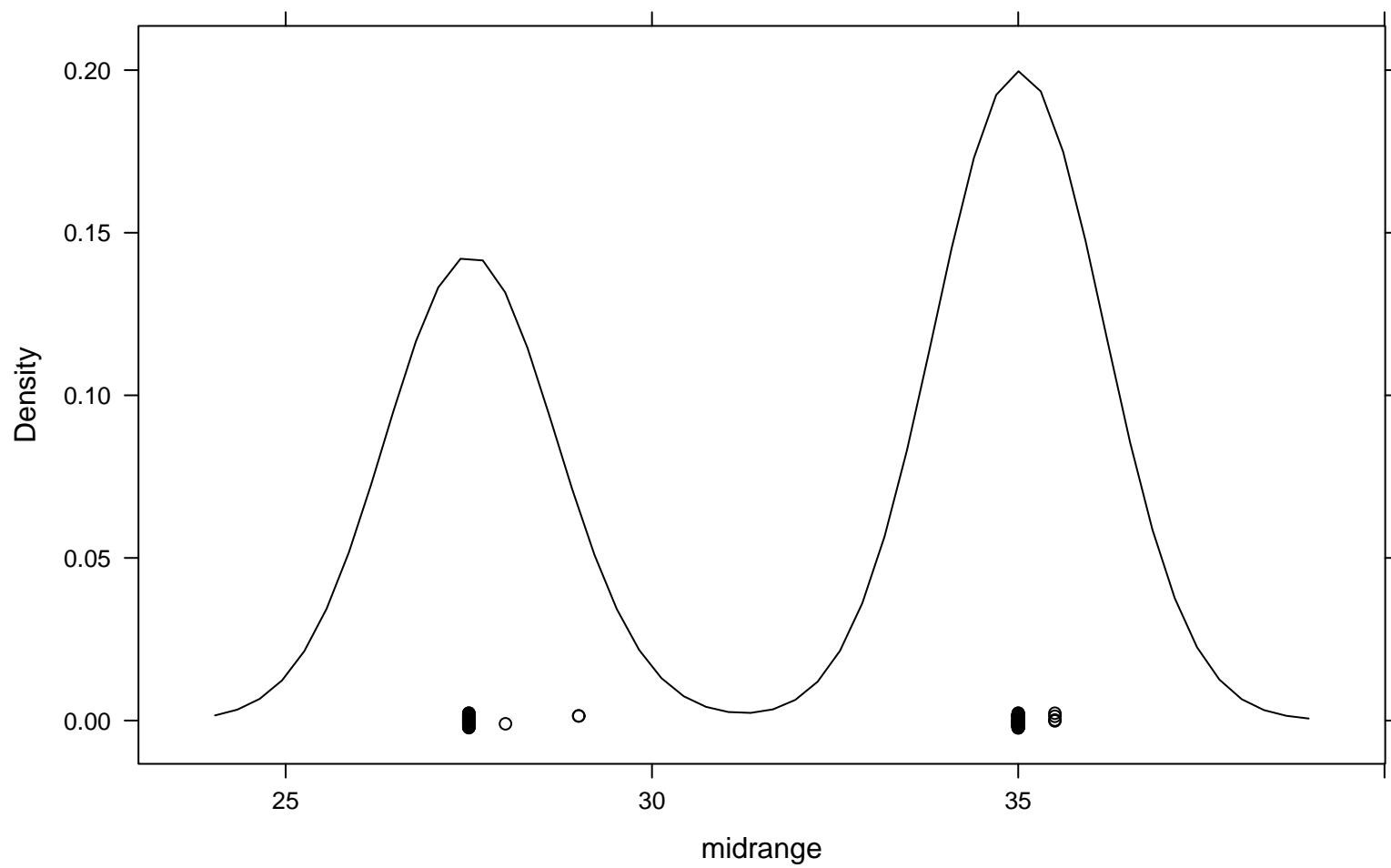
Density Plot
