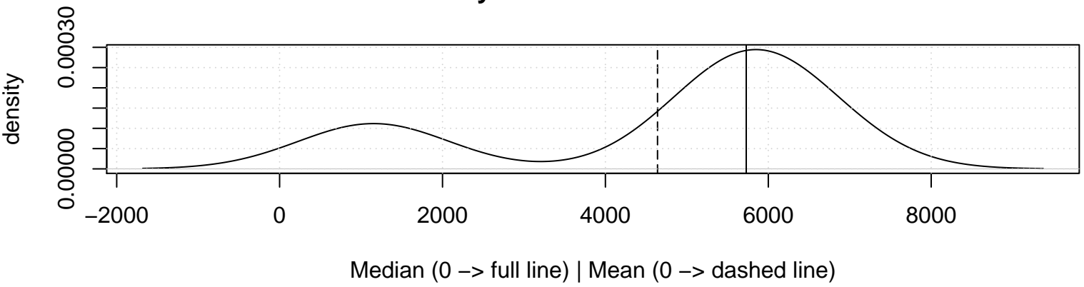
Density Plot – Gaussian Kernel
