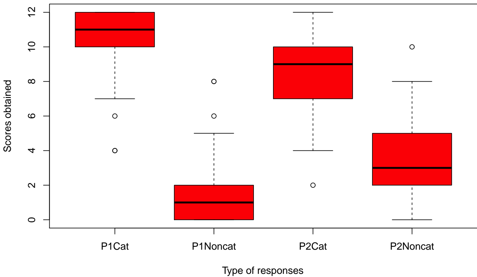
Categorical responses part1 vs part2
