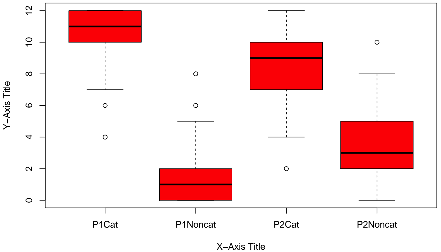
Boxplots Title
