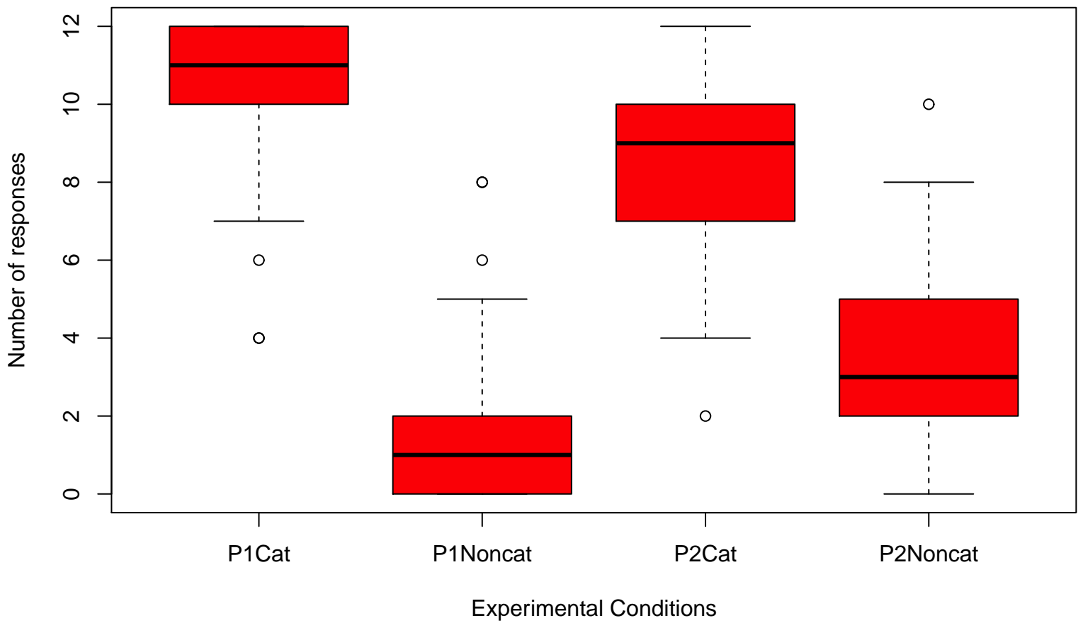
Distribution of scores in each condition
