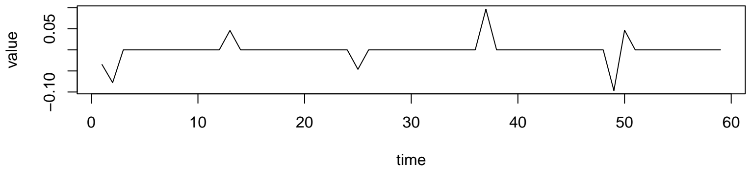
Working Time Series (lambda=0, d=1, D=1)
