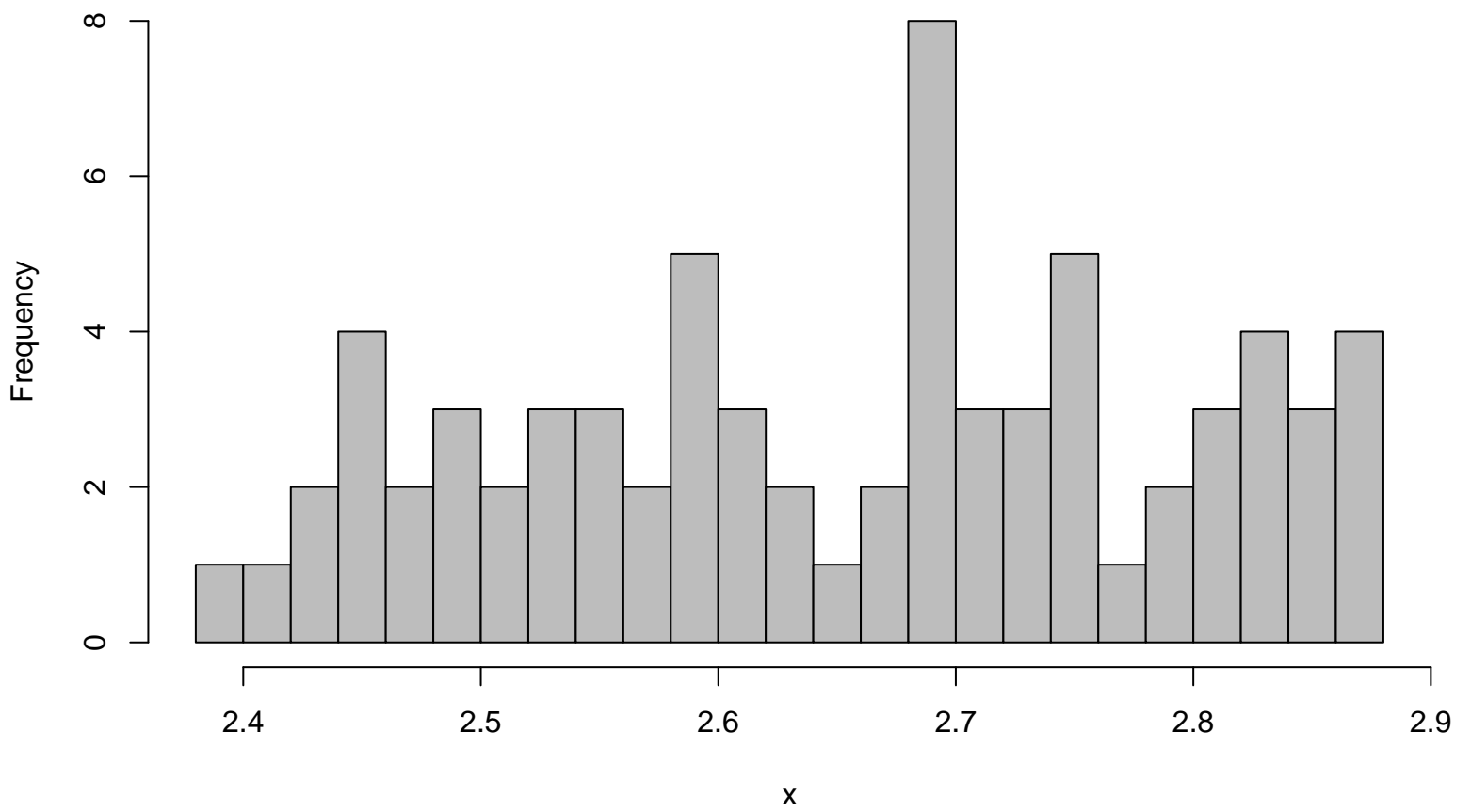
Histogram
