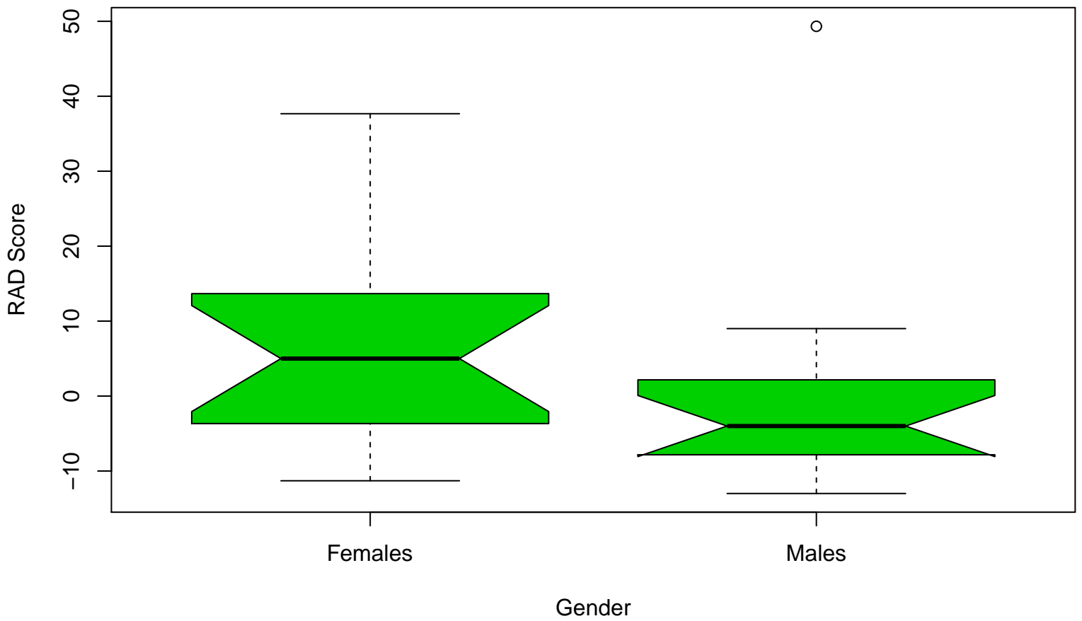
Distribution of female & male RAD scores
