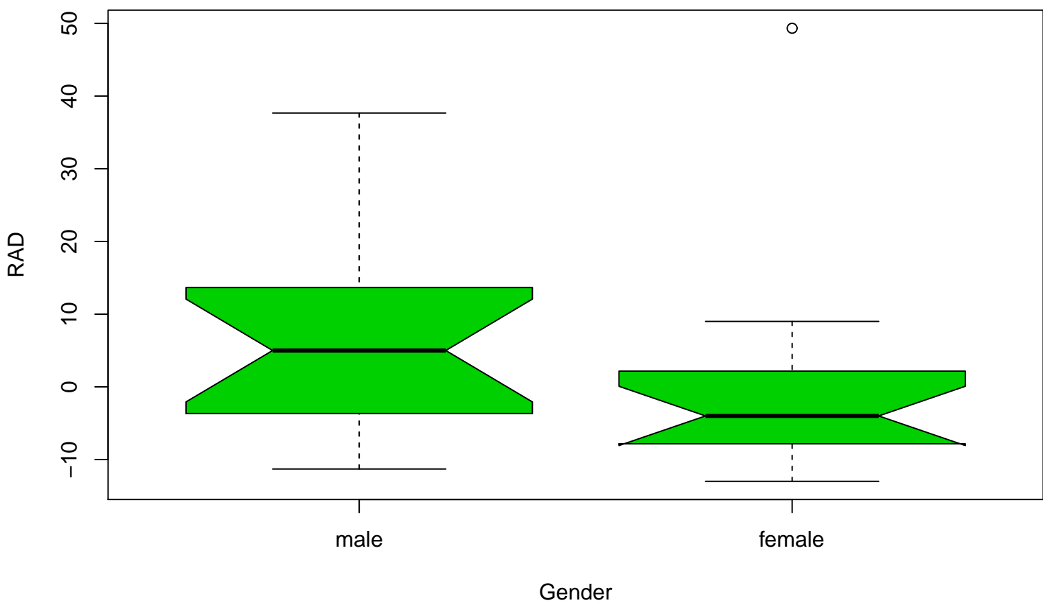
RAD scores
