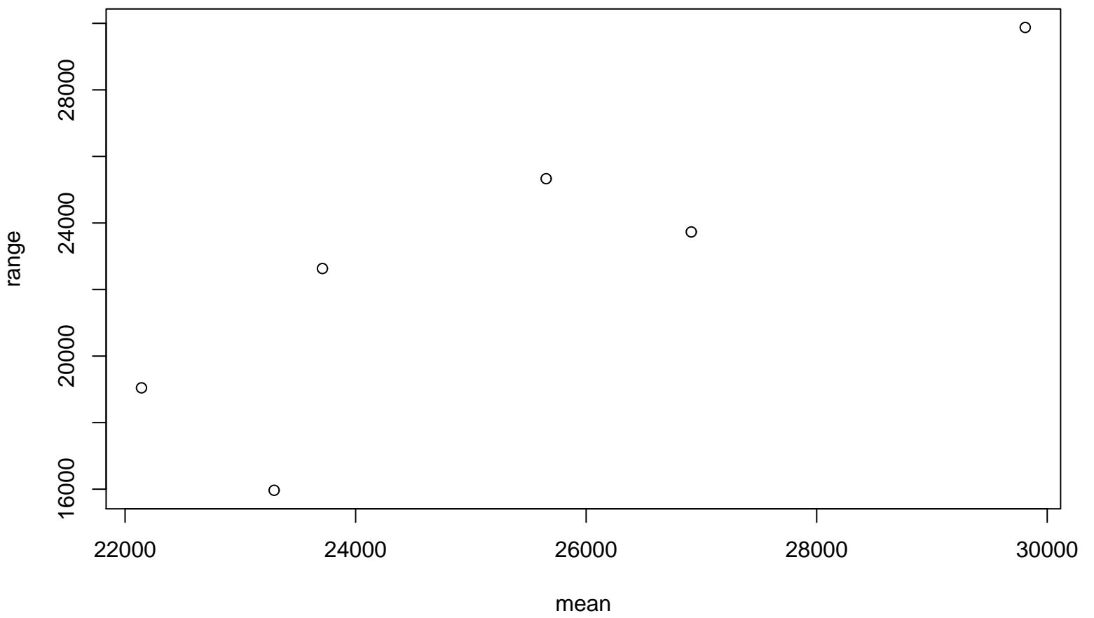
Range-Mean Plot
