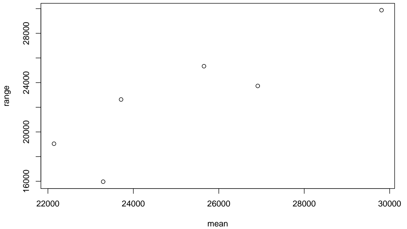
Range-Mean Plot
