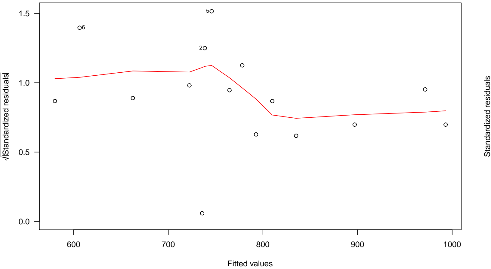
Scale-Location
