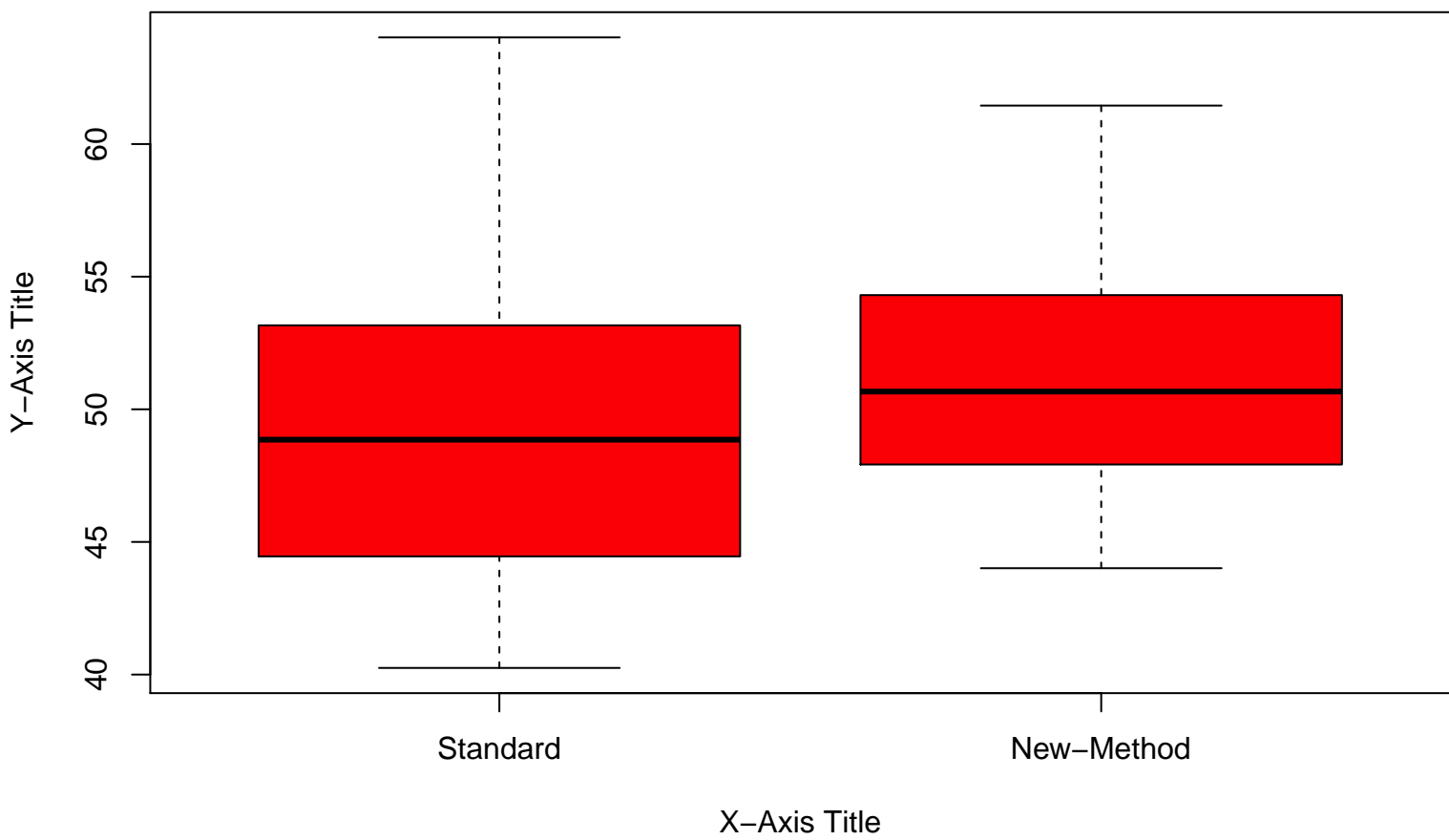
Boxplots Title
