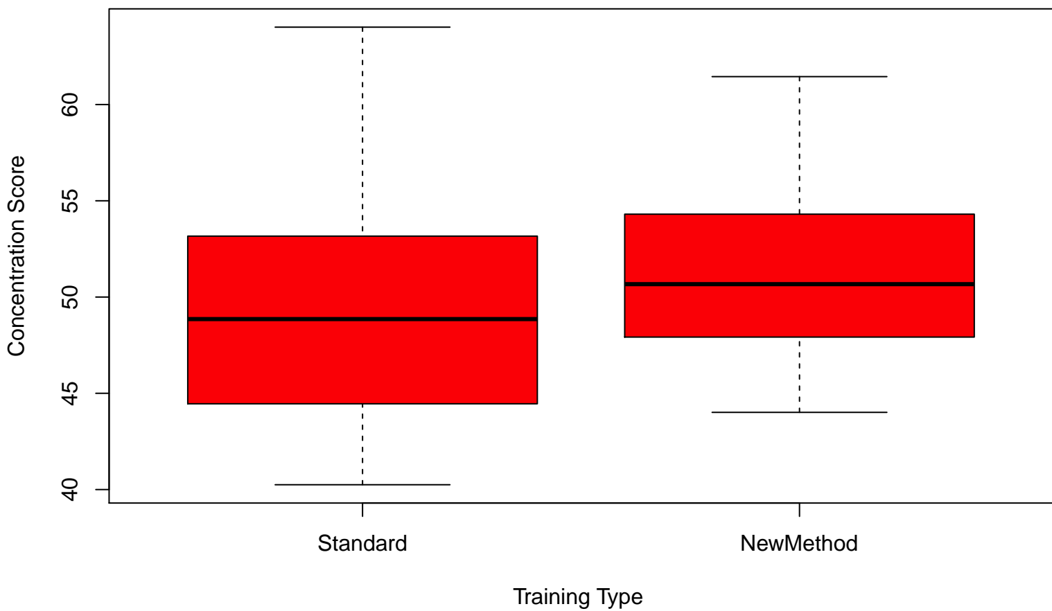
Comparing Concentration Scores achieved
