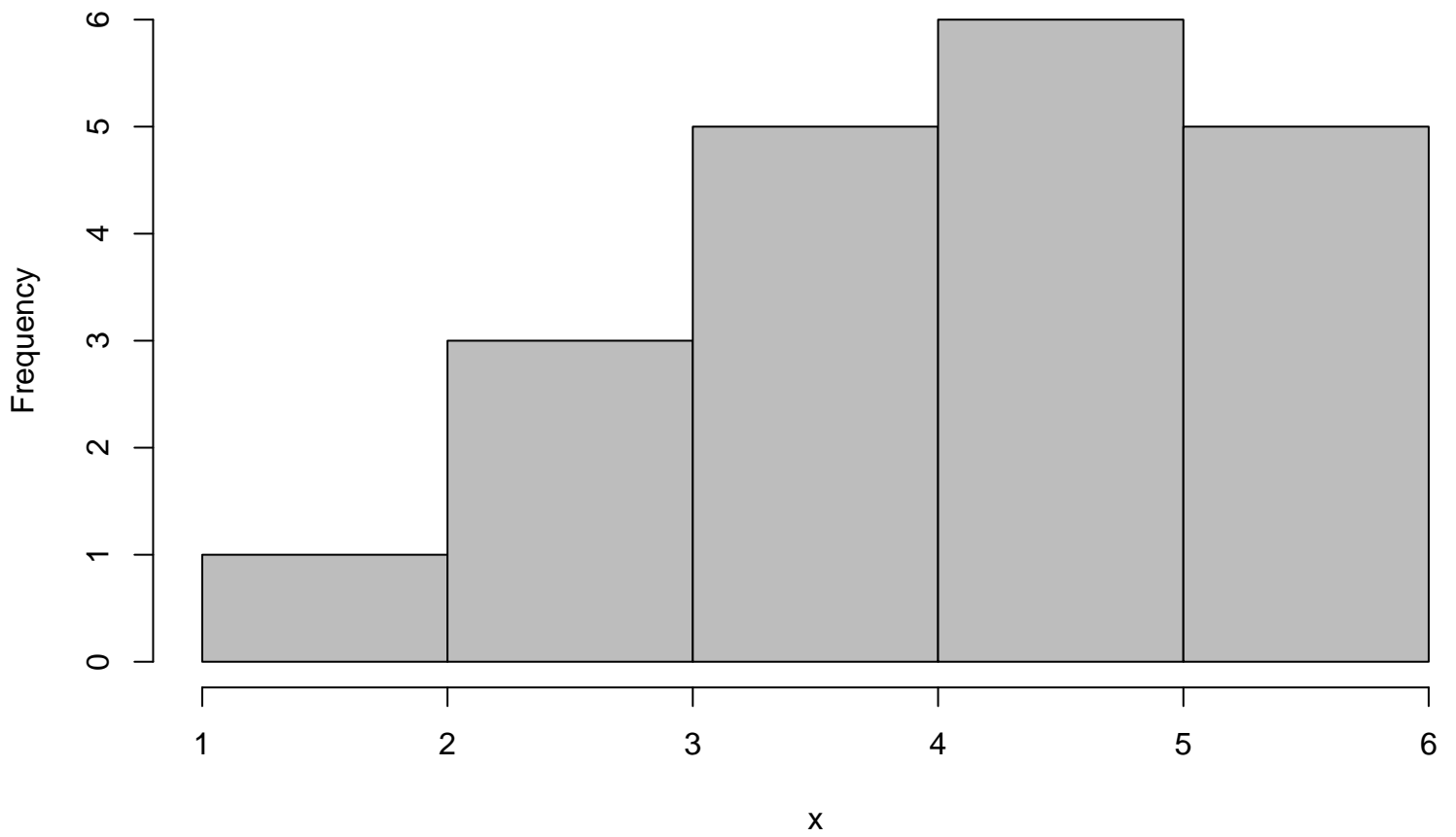
Histogram
