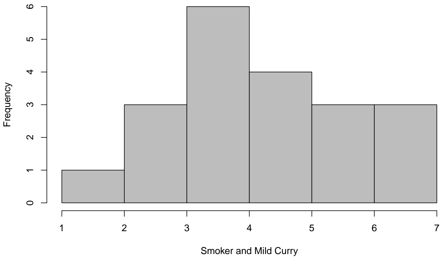
Histogram
