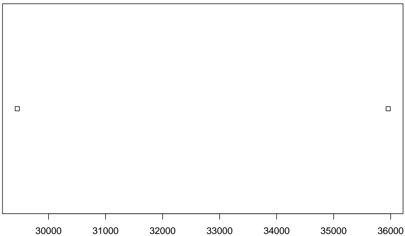
Lag plot (k=7), and lowess
