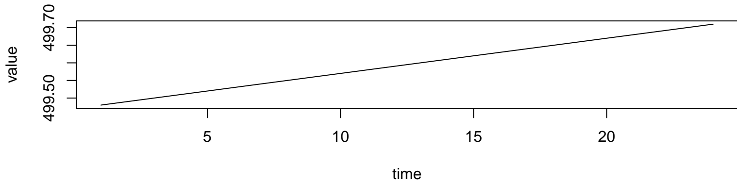
Working Time Series (lambda=1, d=0, D=0)
