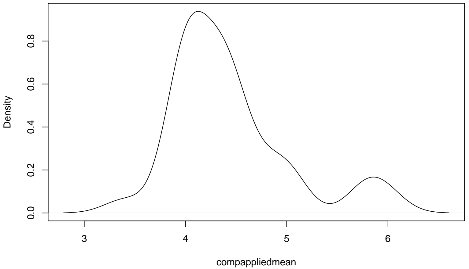
compappliedmean distribution
