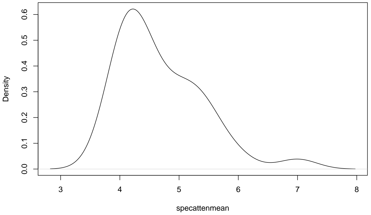
specattenmean distribution
