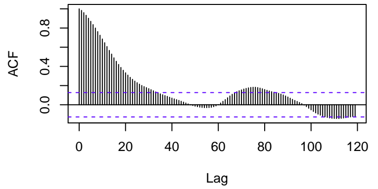
Standardized Residuals
