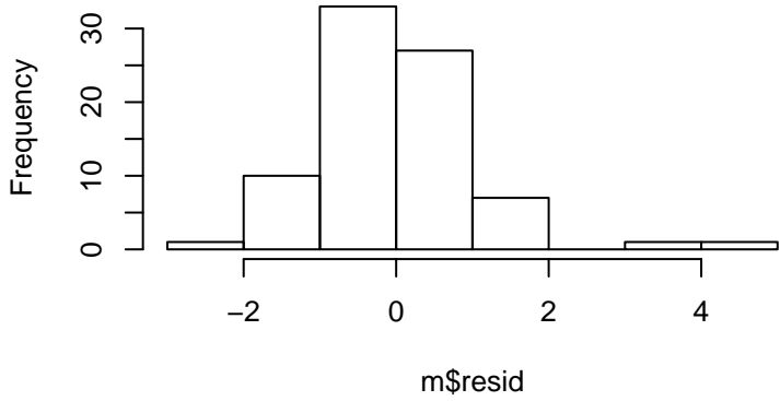
Residual Histogram
