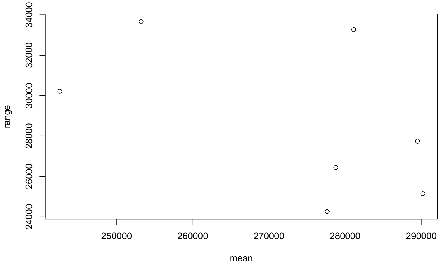
Range-Mean Plot
