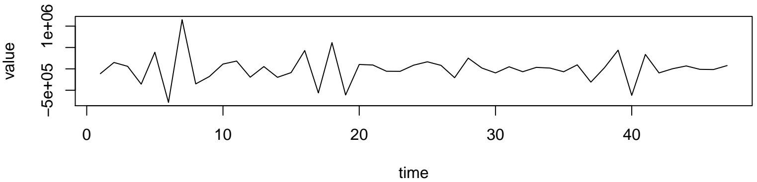
Working Time Series ( \lambda=1 , d=1 , D=2 )
