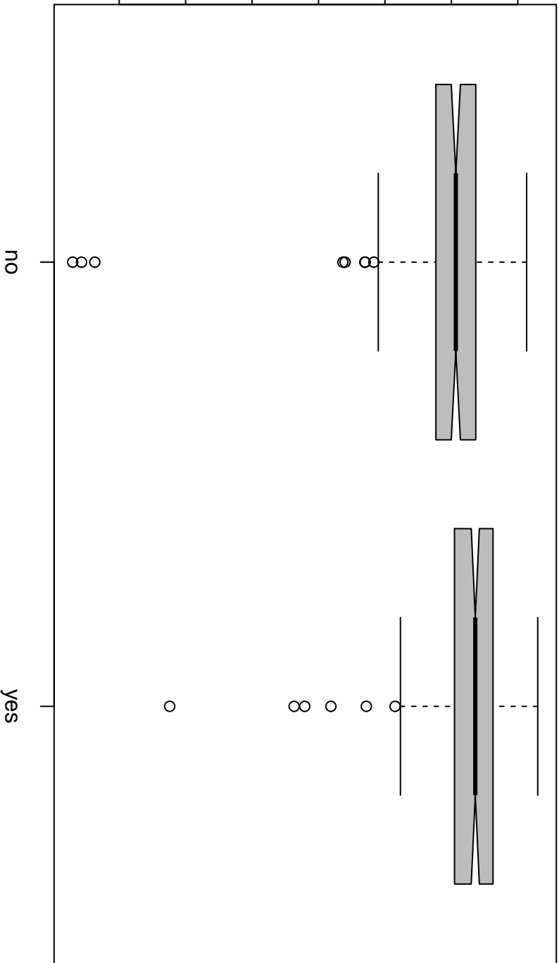
Notched Boxplots
