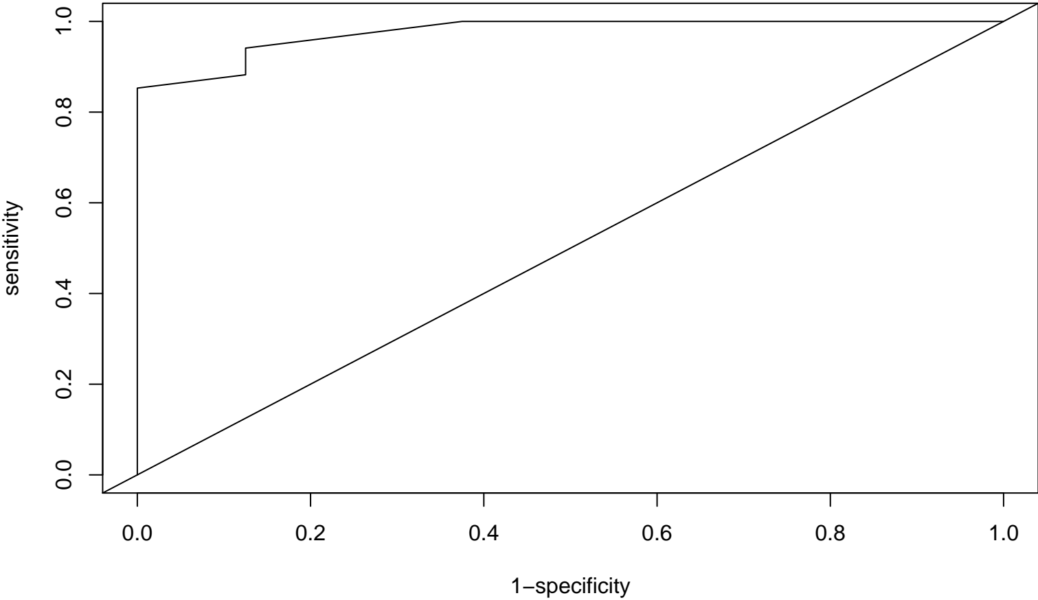
ROC plot
