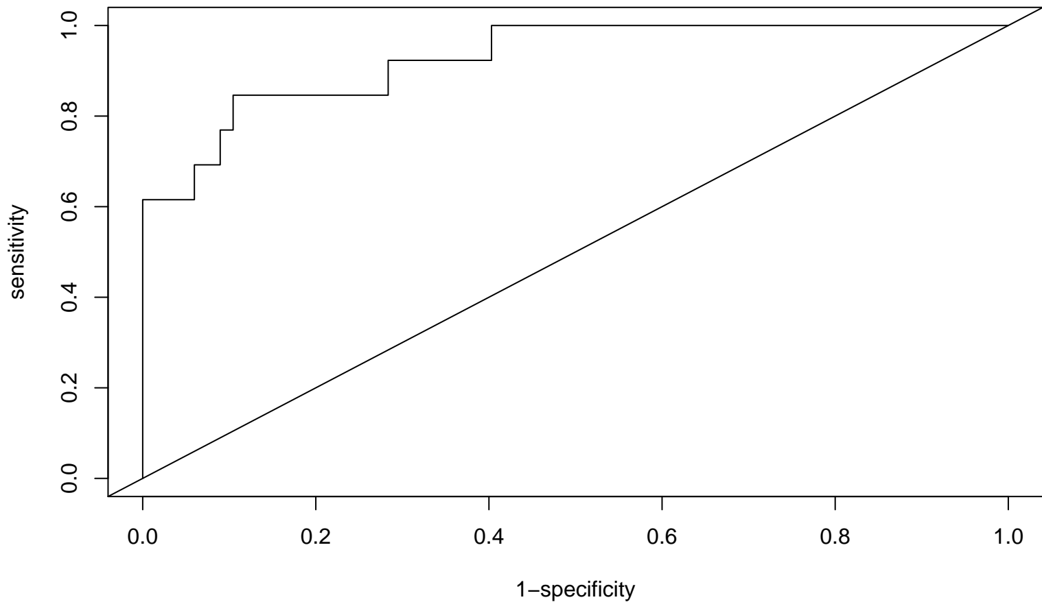
ROC plot
