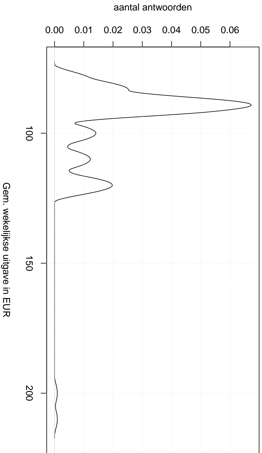
Biweight Kernel
