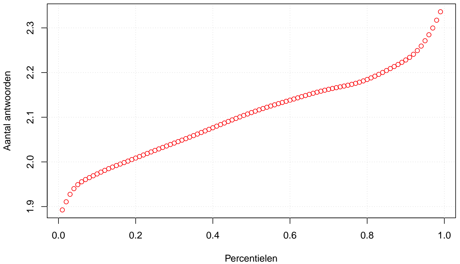
Harrell-Davis Quantiles bananen perc
