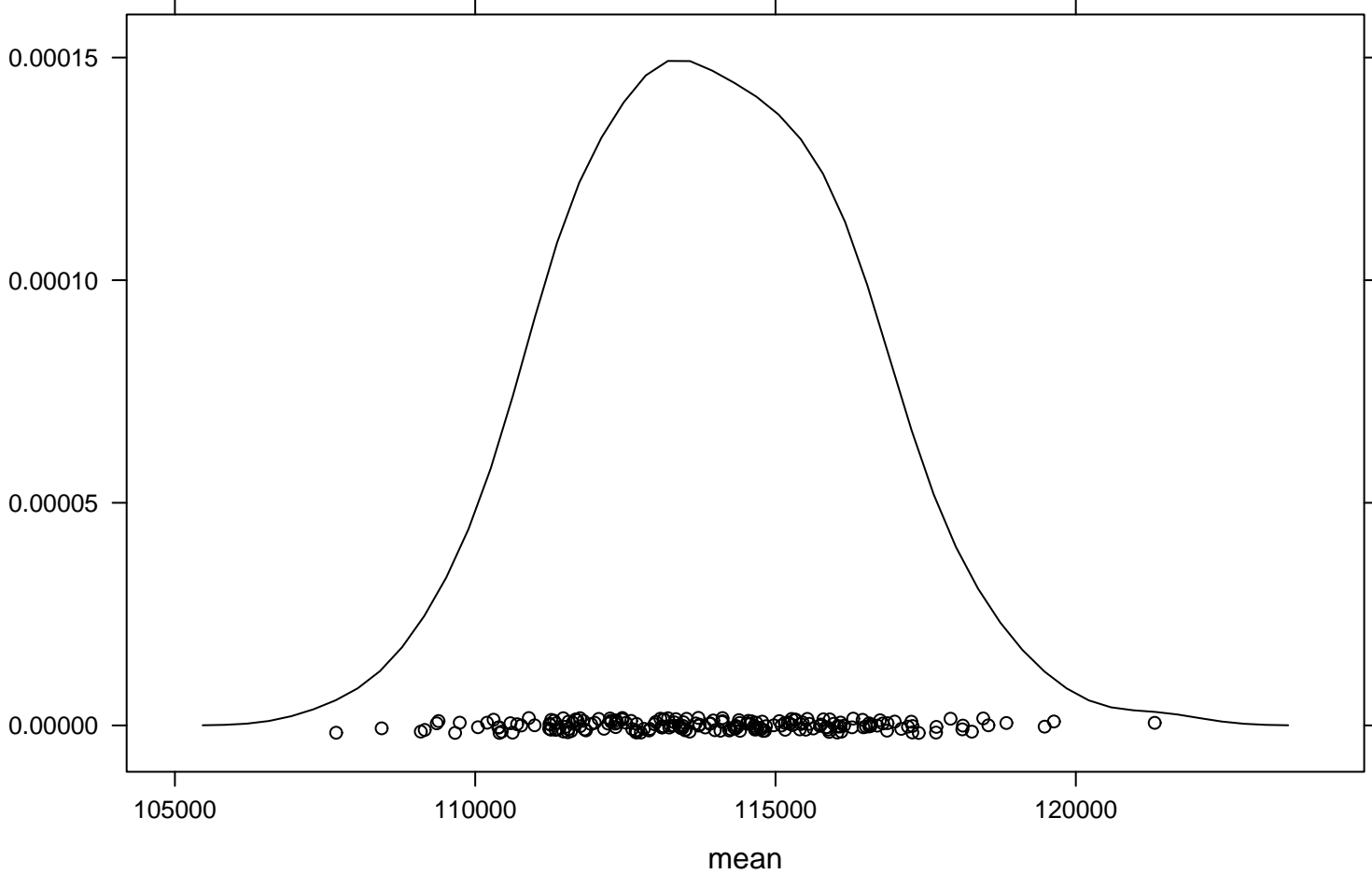
Density Plot
