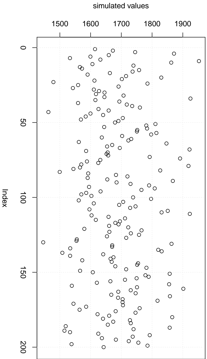
Simulation of Mean
