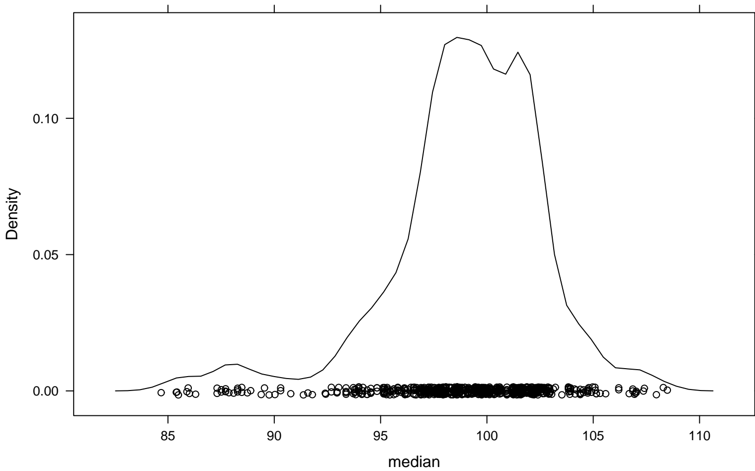
Density Plot
