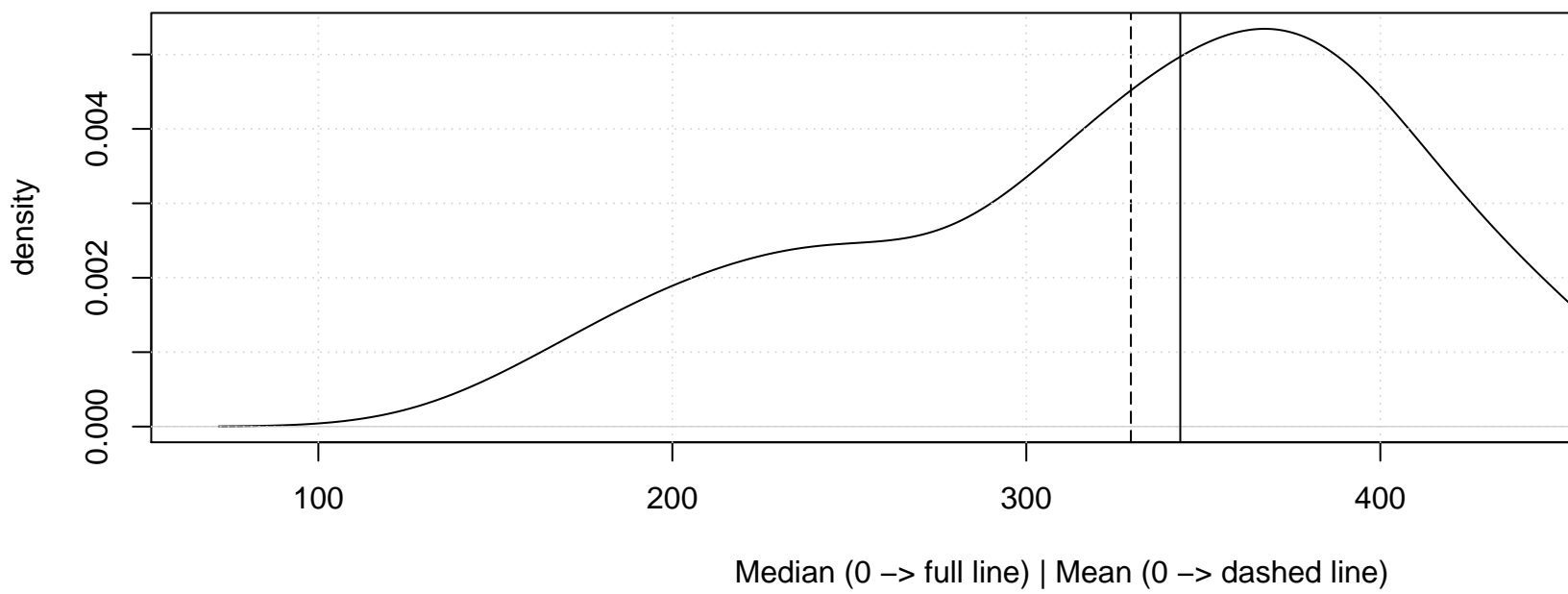
Density Plot – Gaussian Kernel
