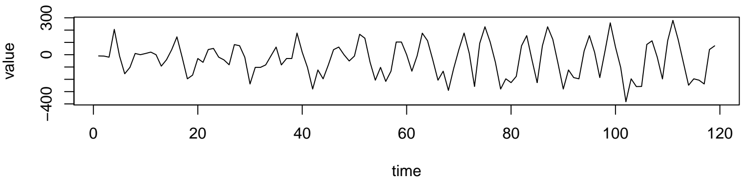
Working Time Series ( \lambda=1, d=1, D=0 )
