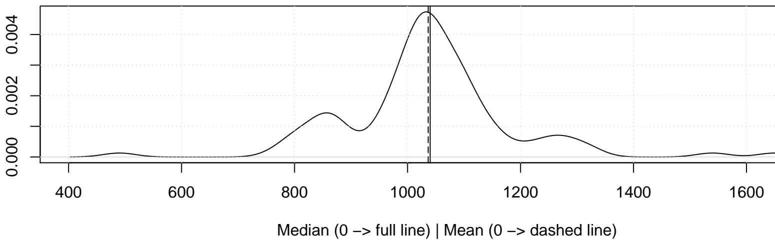
Density Plot – Gaussian Kernel
