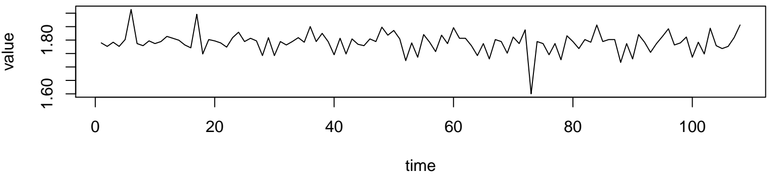
Working Time Series (base=48, d=0, D=0)
