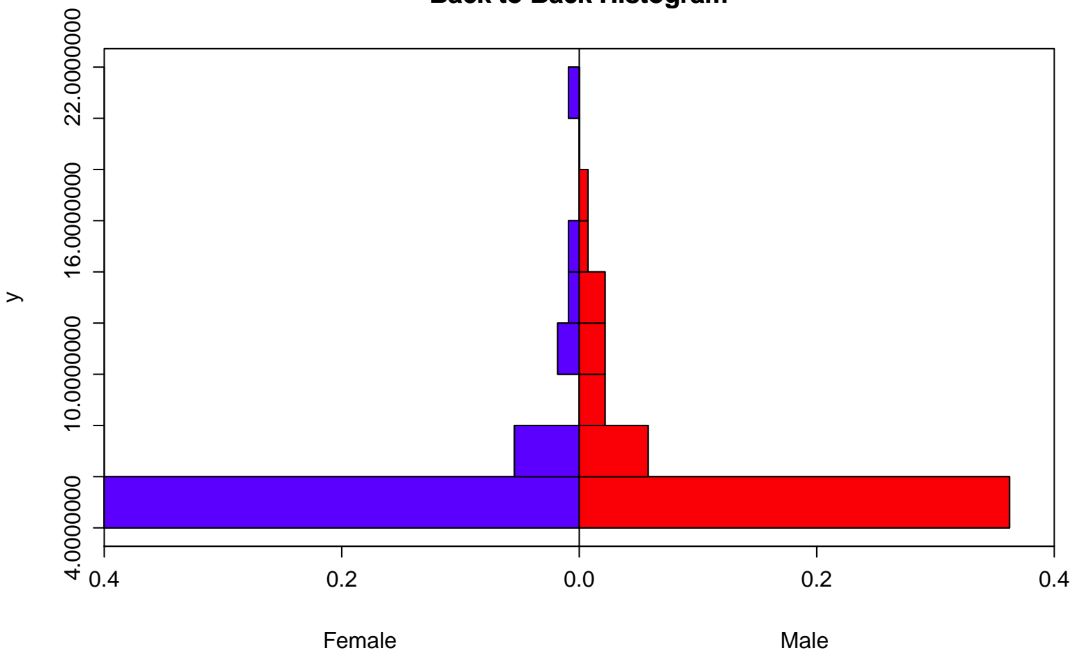
Back to Back Histogram
