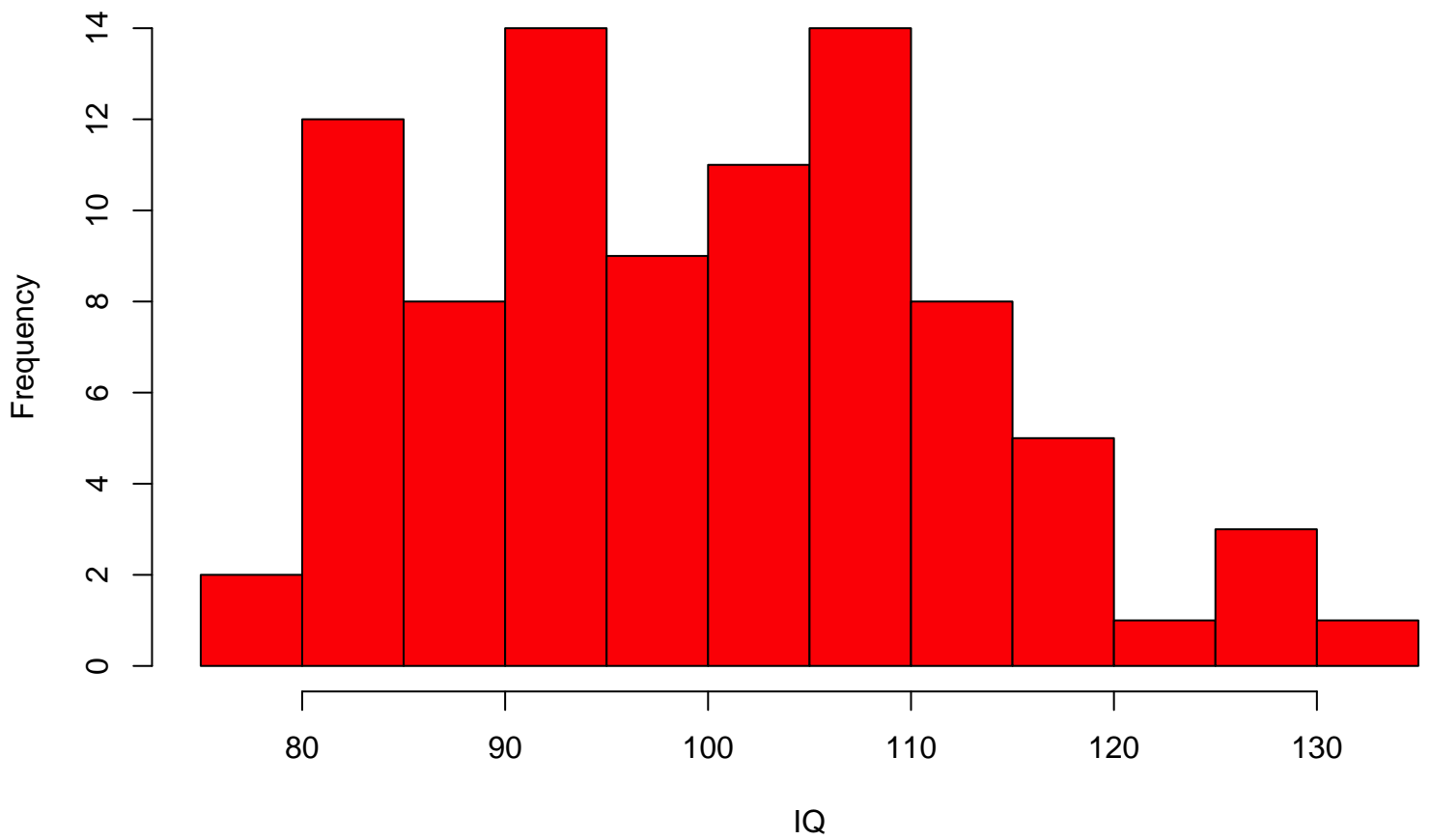
Distribution of IQ
