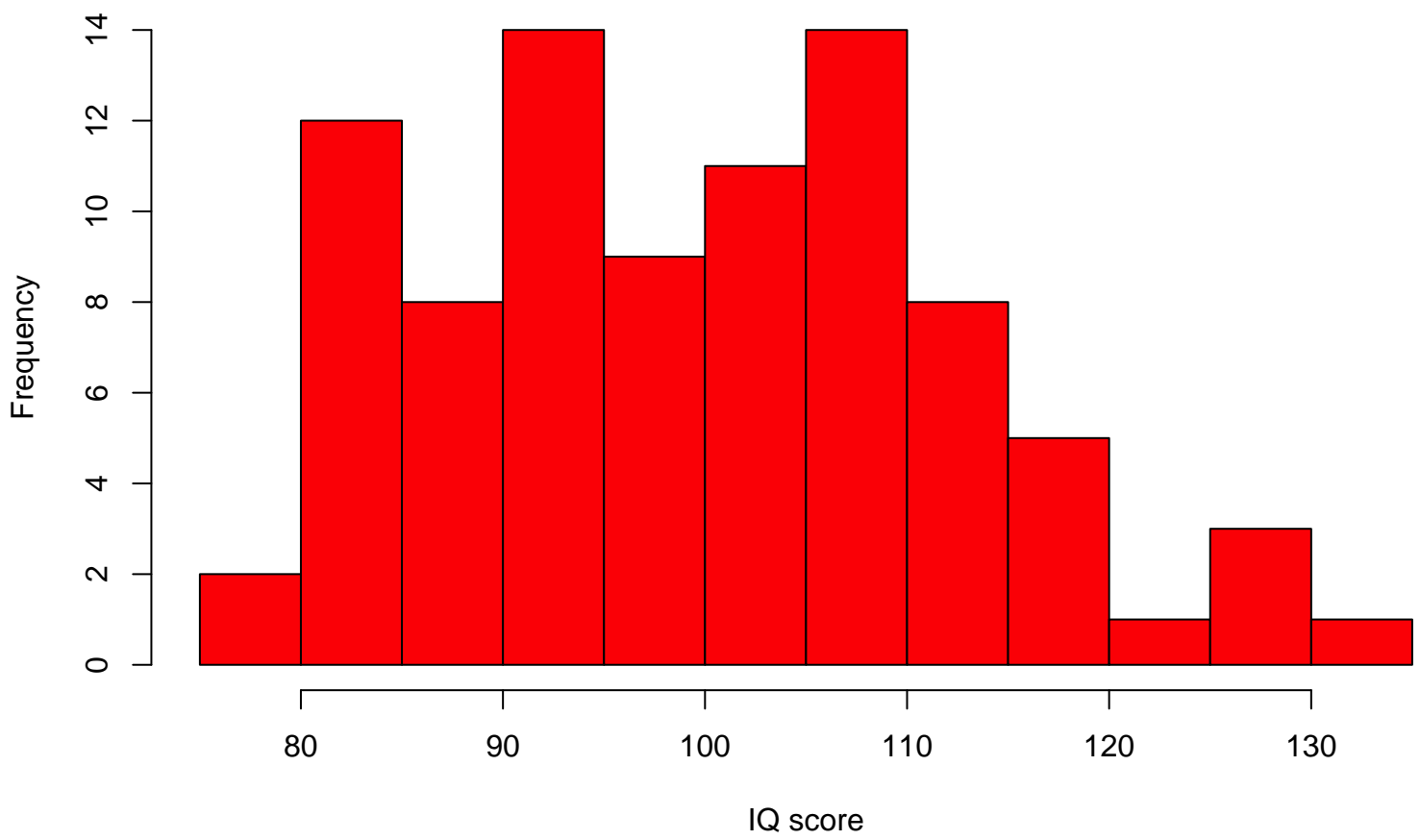
IQ scores
