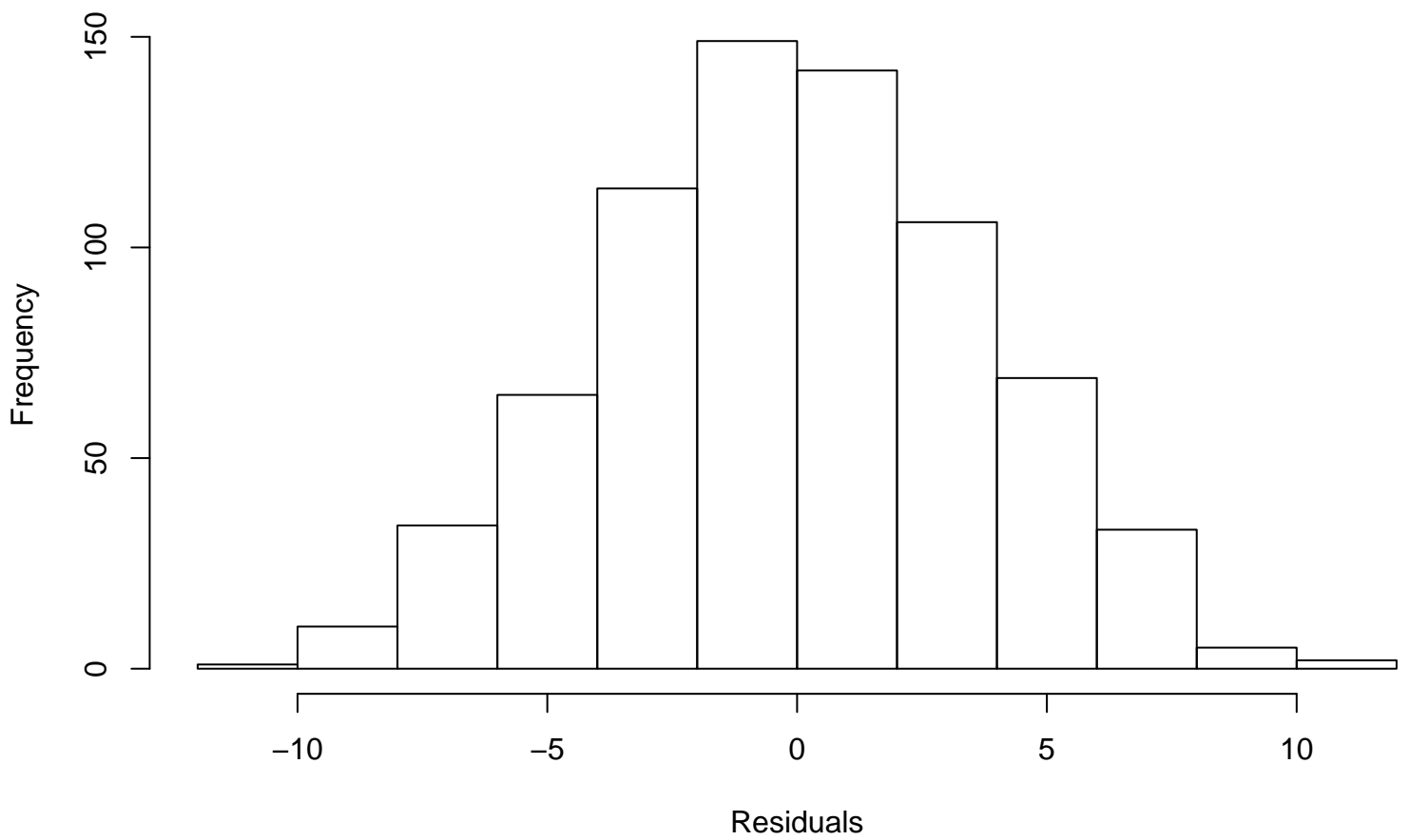
Residual Histogram
