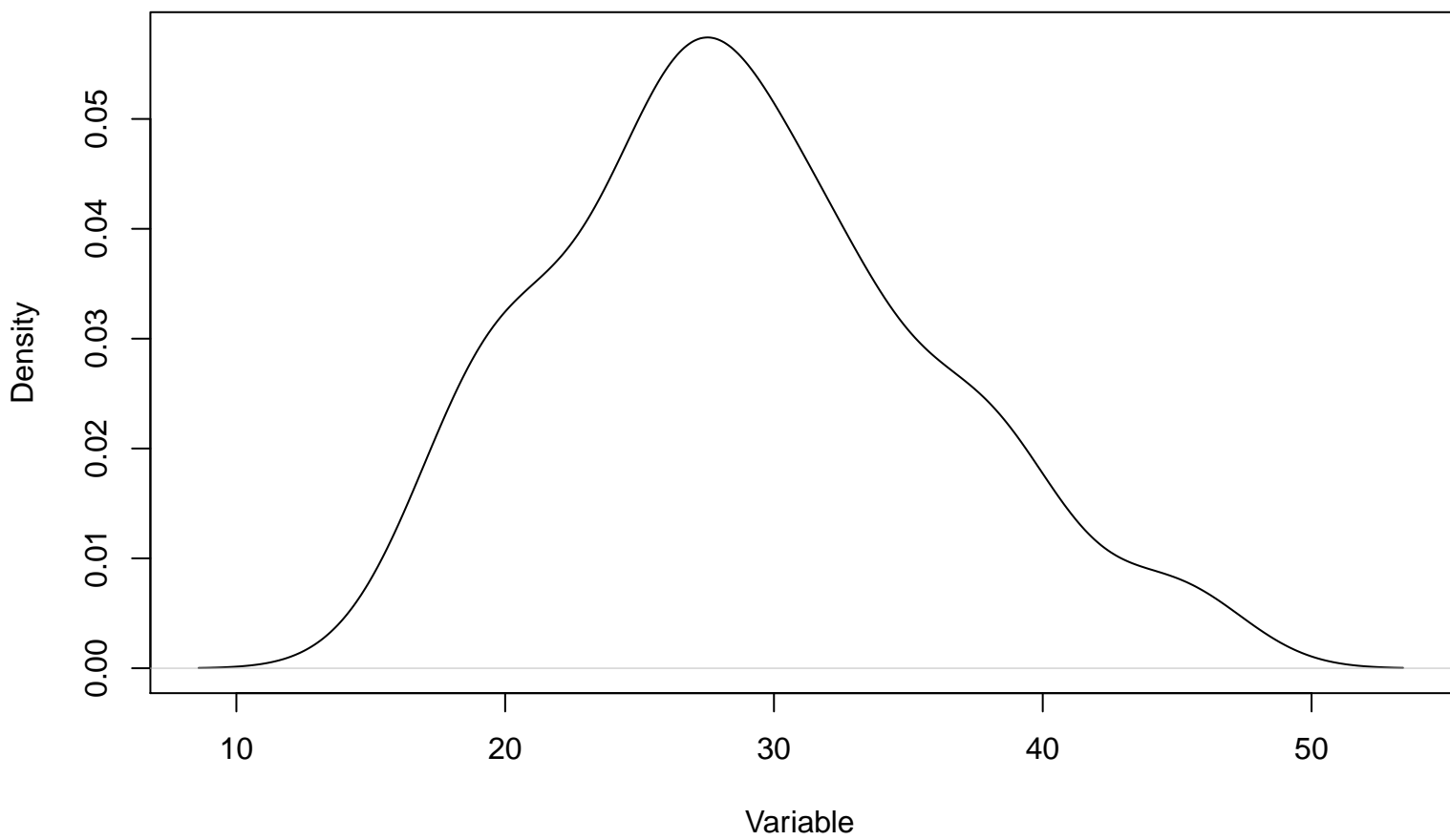
Distributional Plot for distributions
